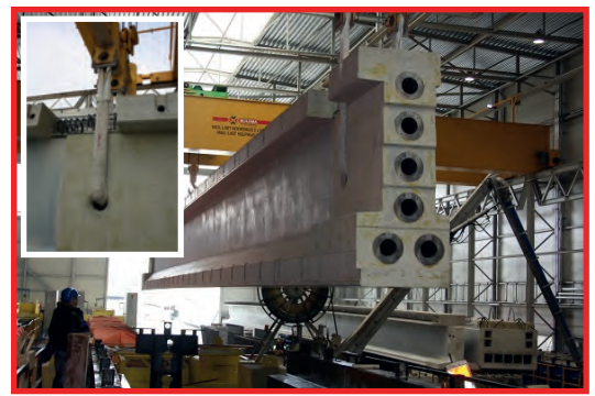
EXTREEMA® CONCRETE MODULE LIFTING MBL 455T
